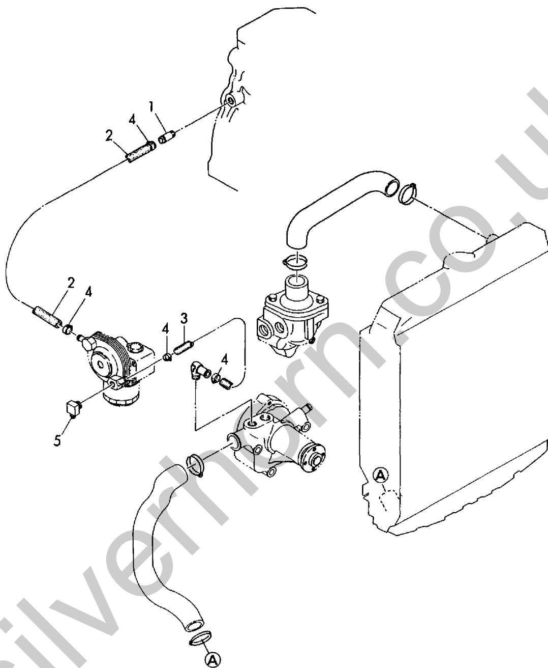
Fig. 31 CWパイプ COOLING WATER LINE
