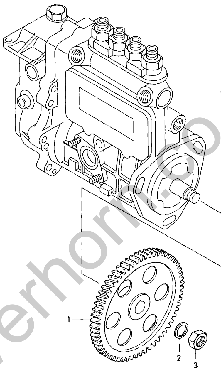
Fig. 19 FOフンシャポンプギヤ FUEL INJECTION PUMP GEAR SPEC. CODE D29150-25200
