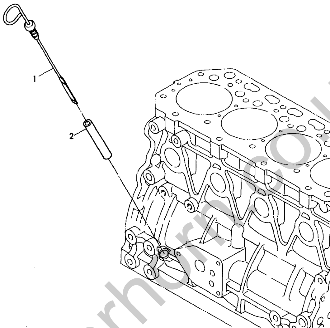
Fig. 22 ケンユボウ LUB. OIL DIPSTICK
